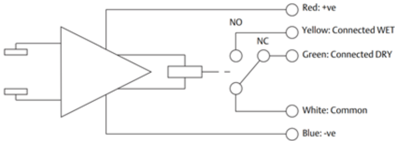
Figure 1. 003S* Schematic
