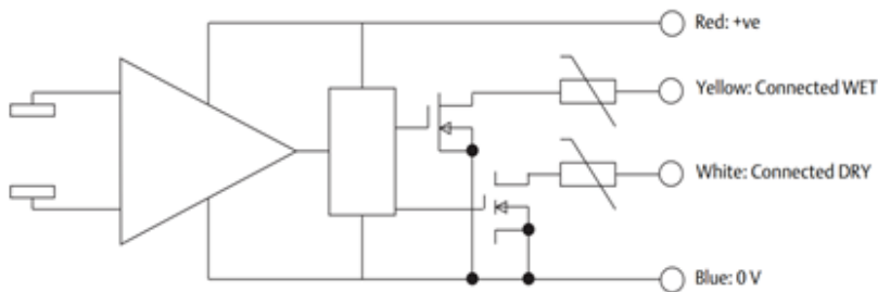
Figure 2. 003H* Schematic
