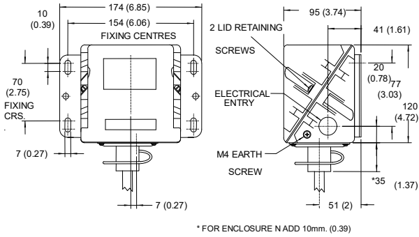
ENCLOSURE W, N
