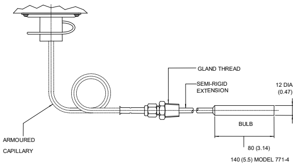
SENSING ELEMENT — MODELS 721, 722, 723, 771, 772, 773 774, 781
